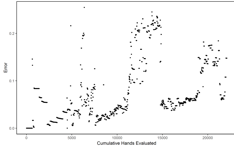
Figure 5: Residuals for Approximation with Tolerance of 0.5
