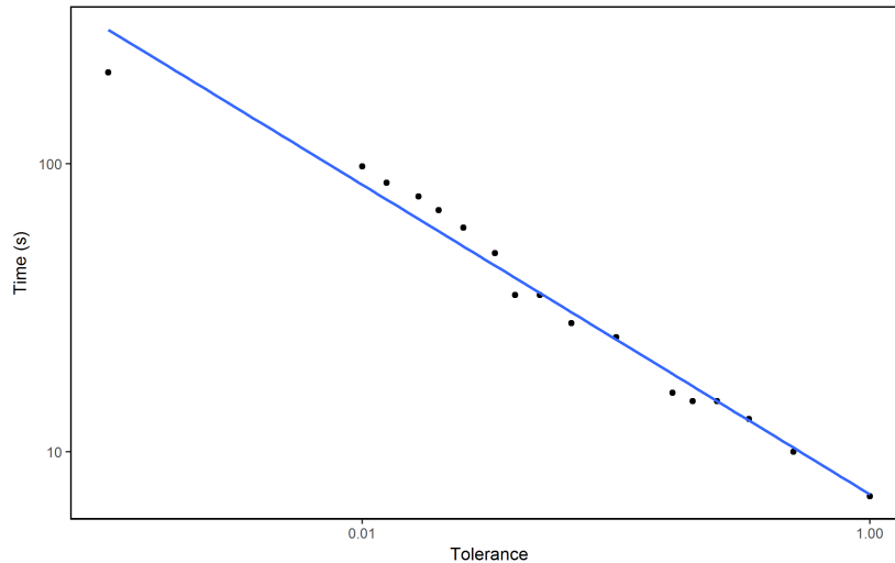
Figure 7: Calculation Time vs. Tolerance (log scales) for 3-Card
