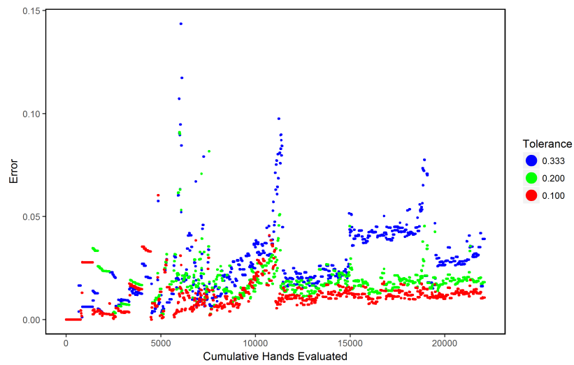
Figure 6: Residuals for Approximations with Various Tolerances
