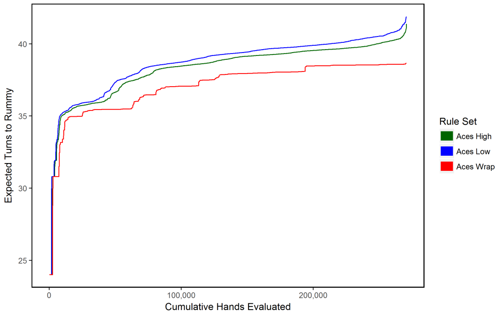
Figure 12: Comparison of Rule Sets for 4-Card Rummy
