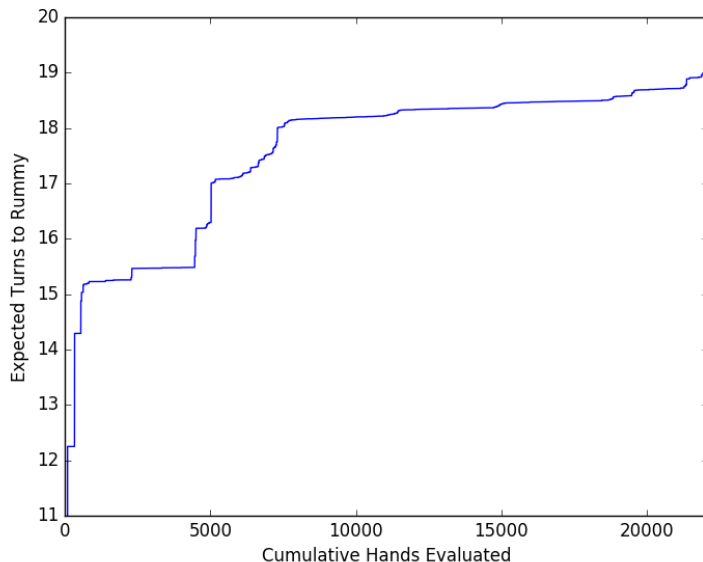
Figure 1: Summary of E for 3-Card Aces Low
