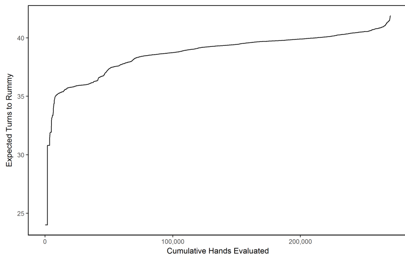
Figure 10: Estimated E for 4-Card Ace Low Rummy with t=0.001
