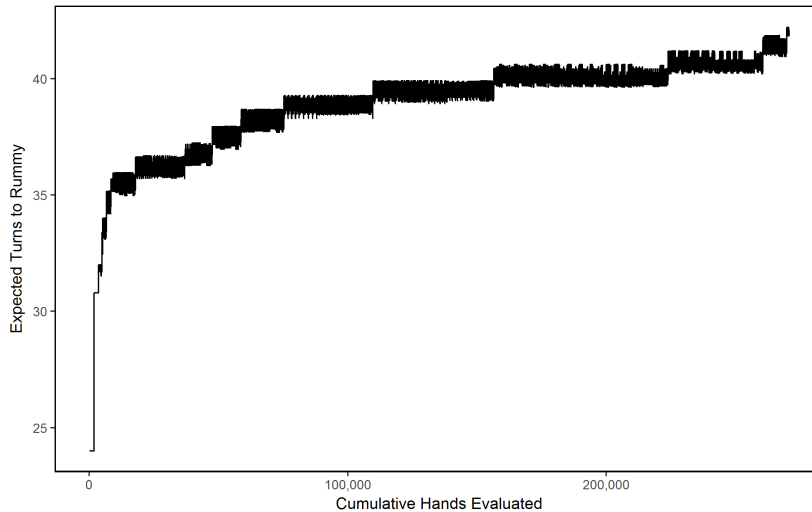
Figure 8: Approximation of E for 4-card Rummy with Tolerance of 1
