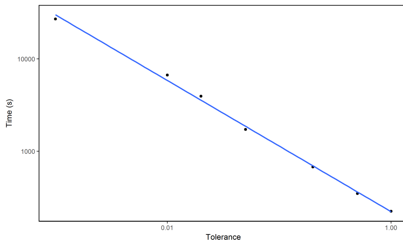
Figure 11: Time vs. Tolerance for 4-Card Approximation
