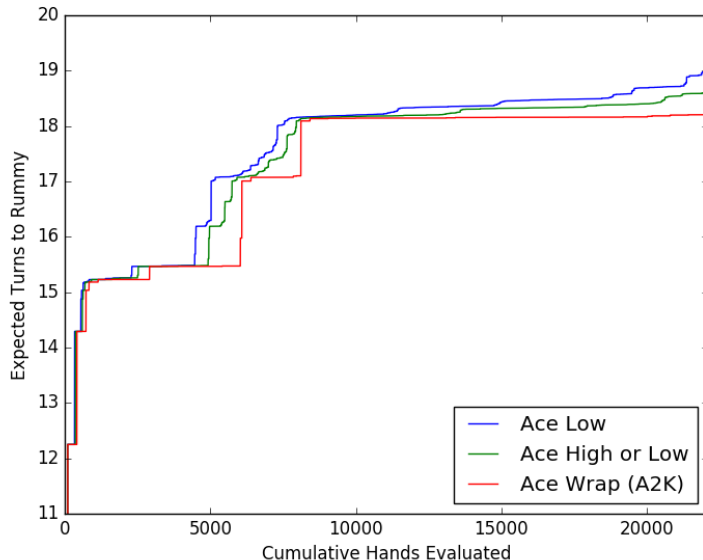
Figure 2: Summary of E for 3-Card Rummy with Various Rules
